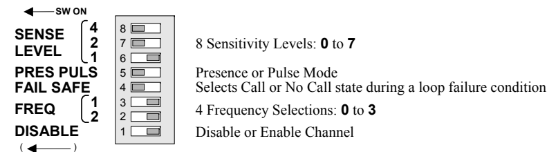
Front Panel Eight-position DIP Switch Module (Factory Default Settings Shown)
