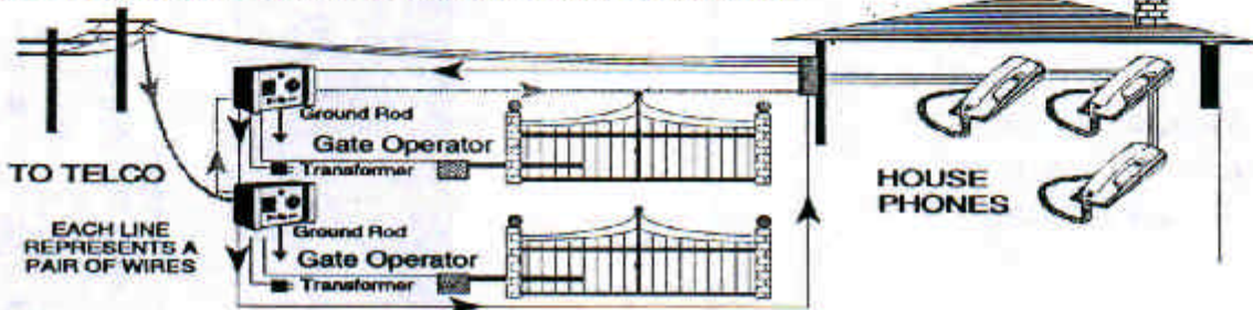
RESIDENCE WITH MULTI-LINE CONFIGURATION W/PBX SG-1 on its own TELCO line.
