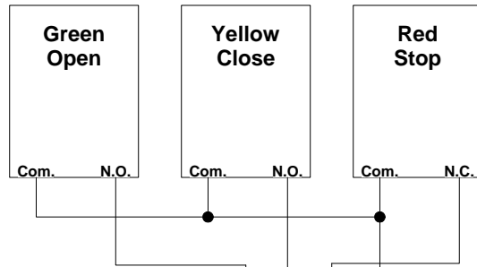
T15 B/C Push Button 3 Button Station
