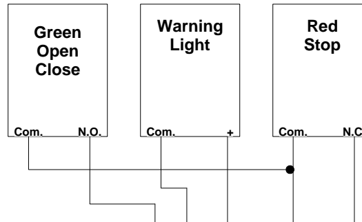
T15 MP Push Button 2 Button Station
