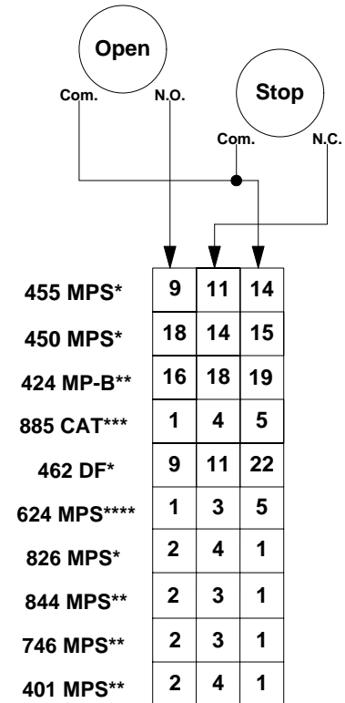
Push Button Switch (indoor)
