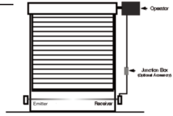
Door Installation
